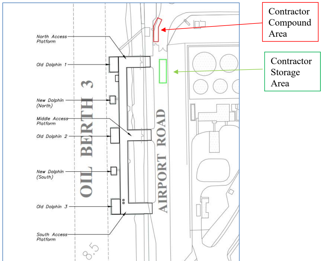
Figure 2: Site Plan
